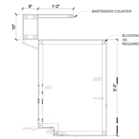
BAR SECTION
